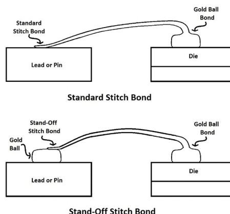
Figure 1. Diagram showing the difference between a SSB and a standard stitch bond.
