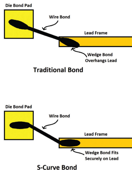
Figure 3. Diagram showing an S-curve bond shape.
