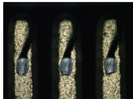
Figure 4. Image of S-curve wire bonds with 125µm pitch.
