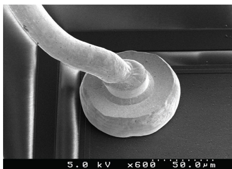
Fatigued/Deformed Wire Bond
