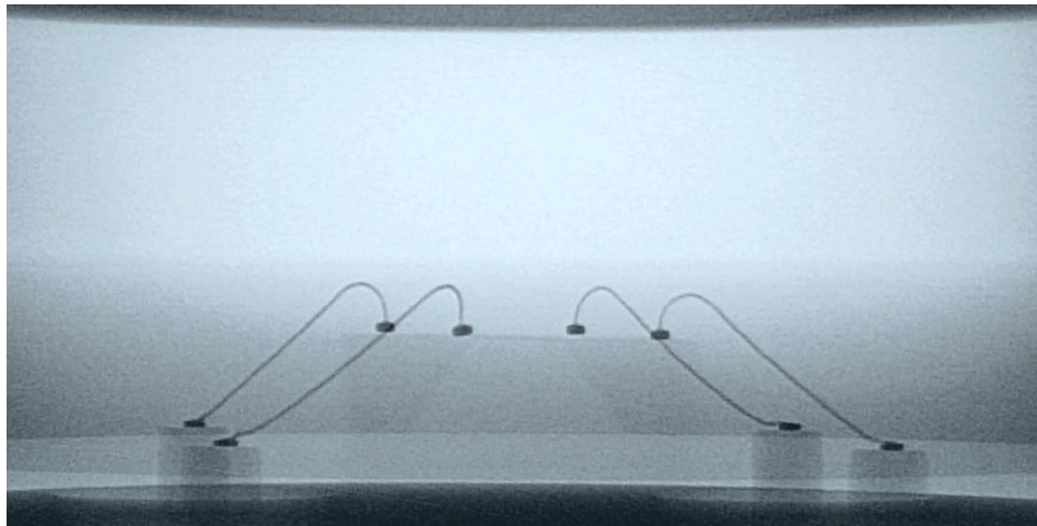
X-ray of Die and Wire Bonds
