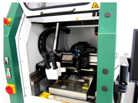
Hesse Mechatronics Model BJ820 Automatic Wire Bonder
