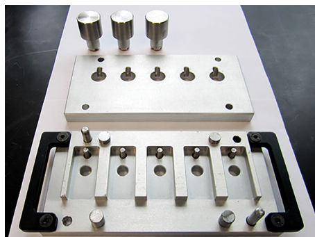
Bottom plate, top plate and weights of the fixture
