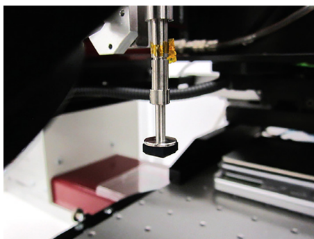
Plastic die attach end-effector makes contact with the parts being assembled.
