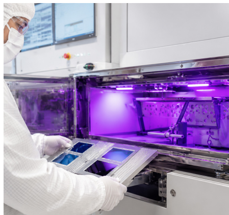
SMART Microsystems' Super Ultraviolet (SUV) Accelerated Test Chamber is one of only three in the U.S. providing access to a unique and valuable capability.
