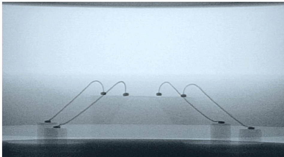
Figure 1. X-ray of die and wire bonds after gel dispense.
