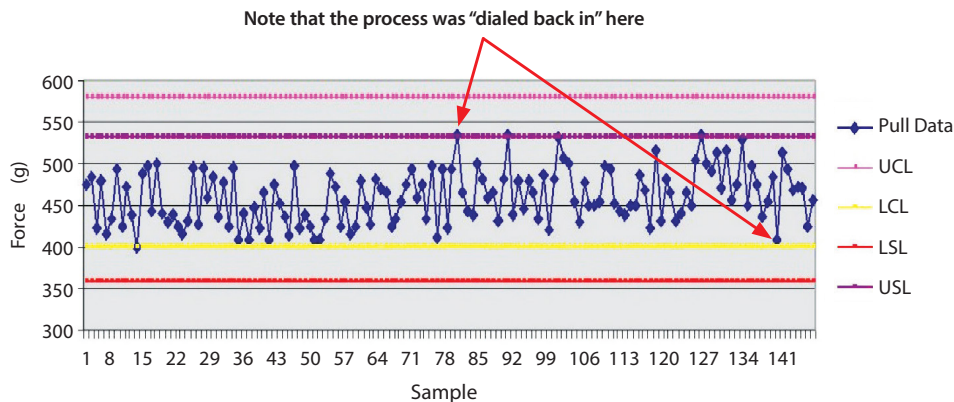
Figure 2. Example of early SPC data collected for a real wire bond process
