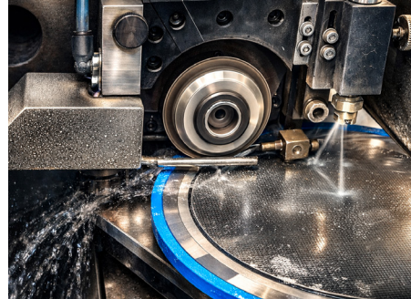
Figure 3. Typical wafer dicing environment
