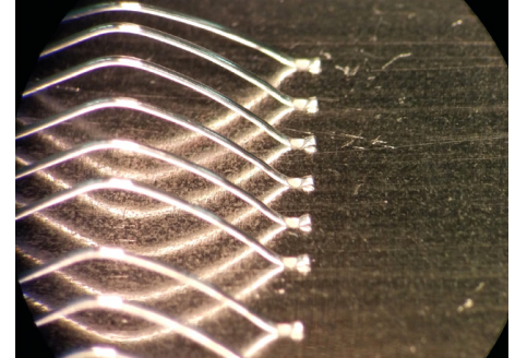
Figure 5. Aluminum wire bonds
